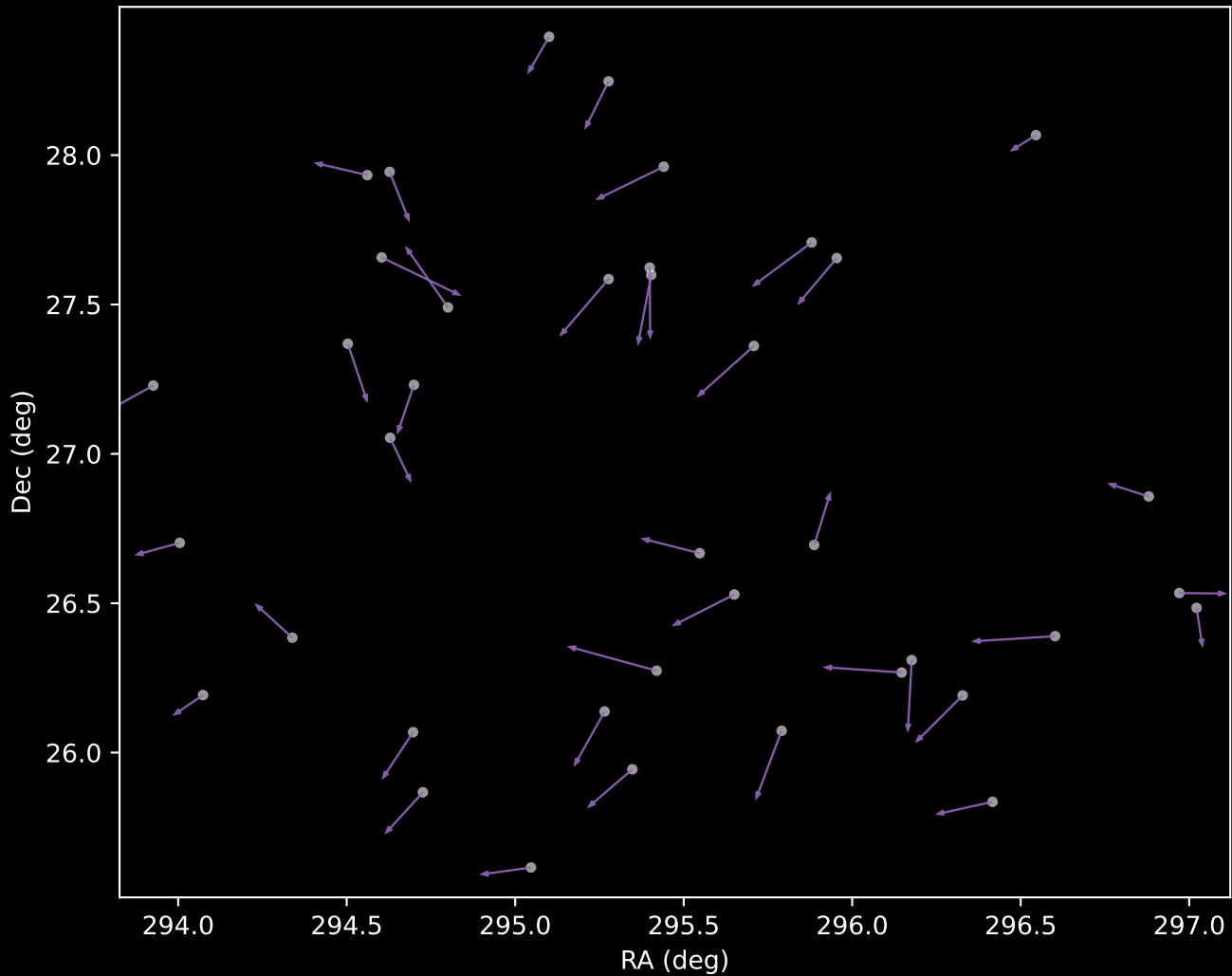
APOGEE DR17 Cluster 8 Proper Motion Vectors (n=39)
