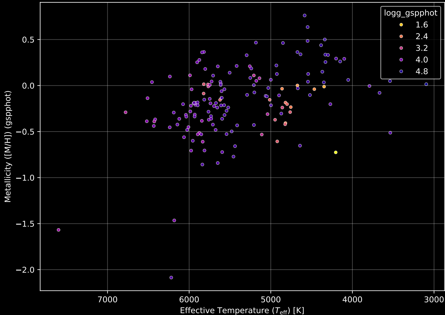
APOGEE DR17 Field: [029+88_MGA] Stellar Population Parameters (n= 157)
