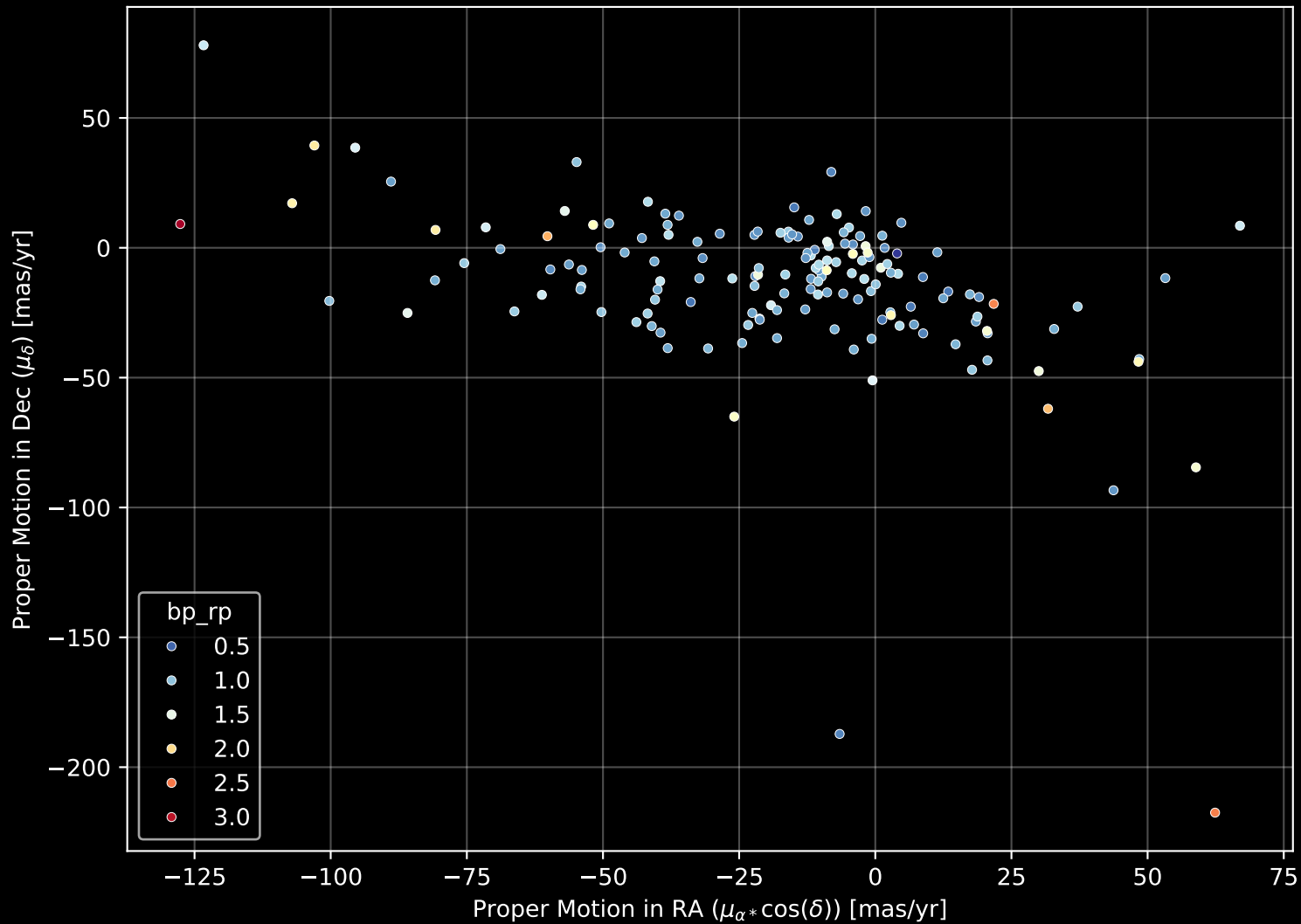
APOGEE DR17 Field: [029+88_MGA] Proper Motion Diagram (n= 157)
