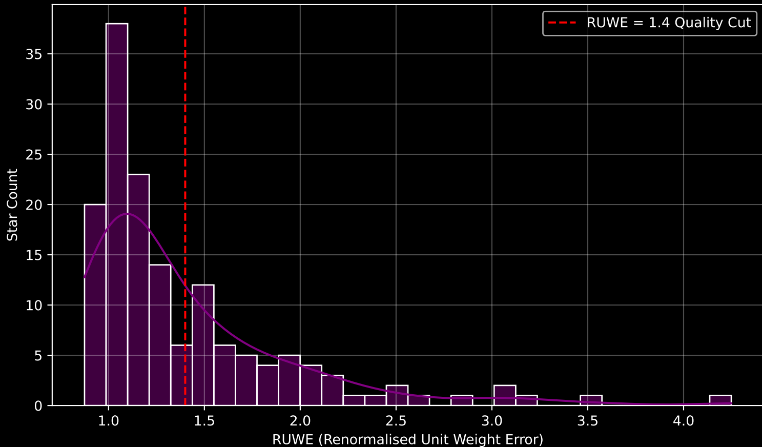
GAPOGEE DR17 Field [029+88_MGA] RUWE Distribution (n= 151)
