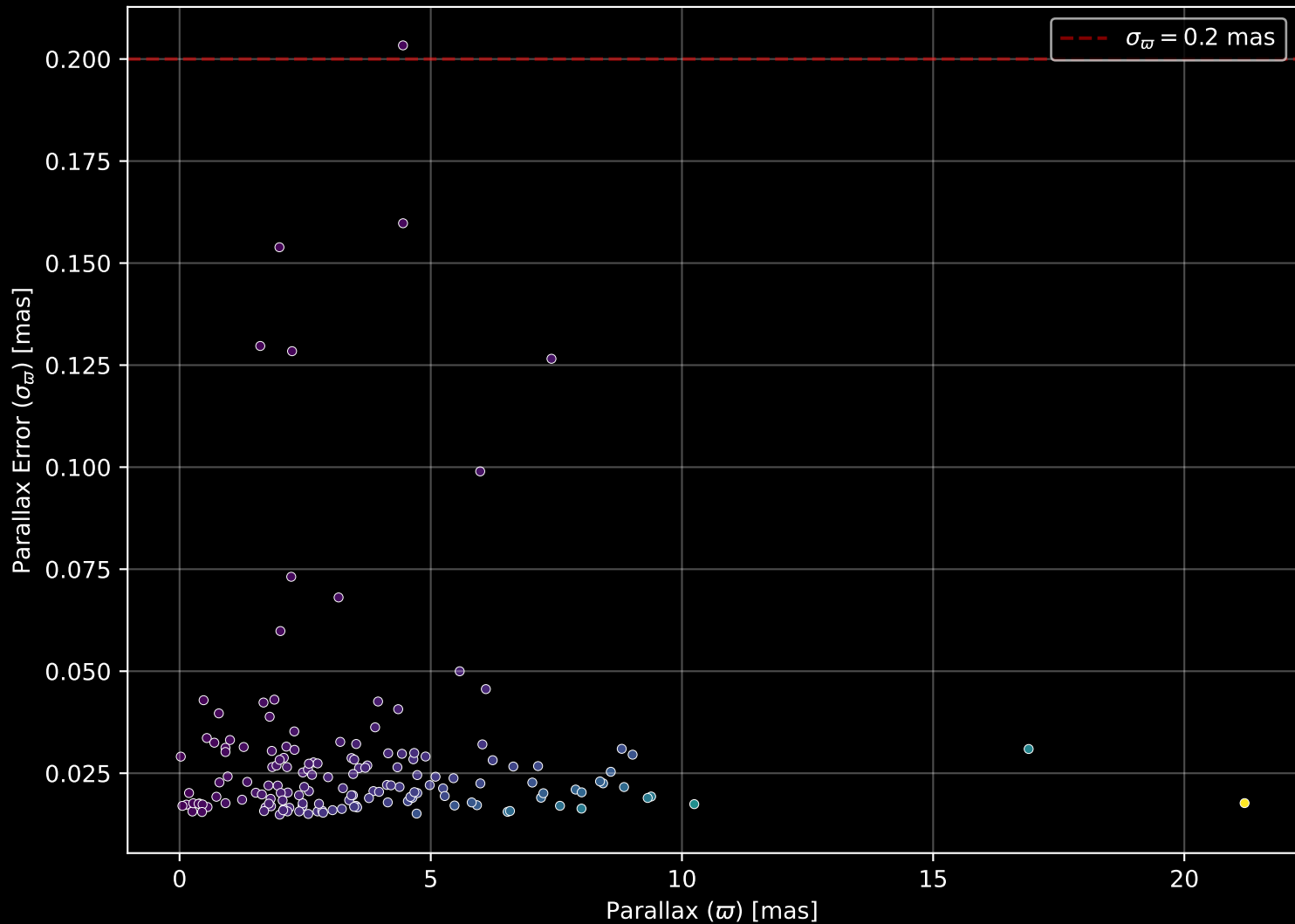
APOGEE DR17 Field: [029+88_MGA] Parallax Quality (n= 157)
