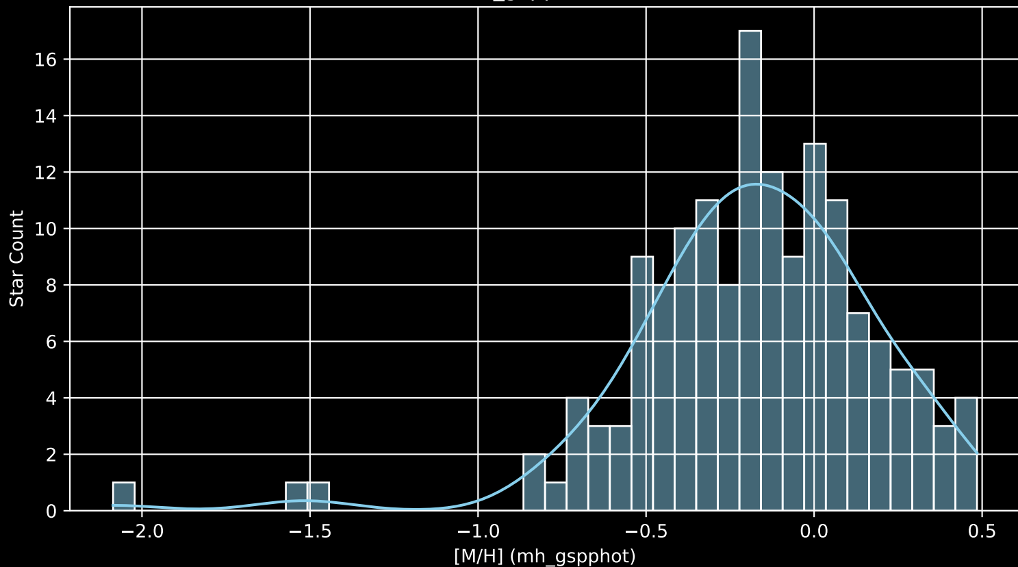
APOGEE DR17 Field: [029+88_MGA [M/H] (mh_gspphot) (n= 154)
