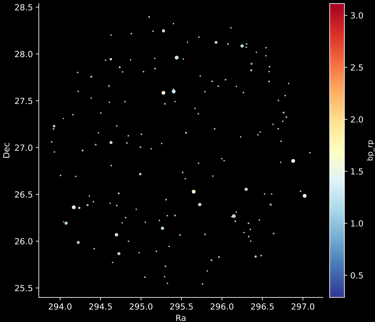
APOGEE DR17 Field: [029+88_MGA] Stars: 157
