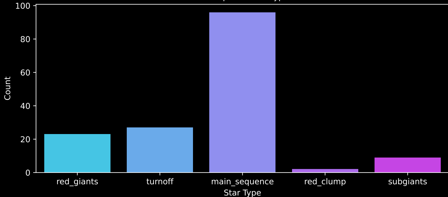
APOGEE DR17 Field: [029+88_MGA] Count plot of Star Type
